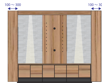
W2018 ~ 2418 D470 H1792 mm
